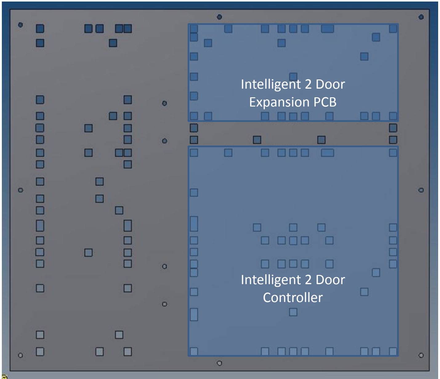
PCB Mounting Options
